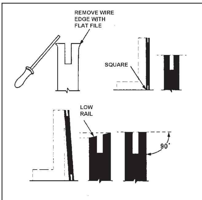
Figure 7. Rail Wear
