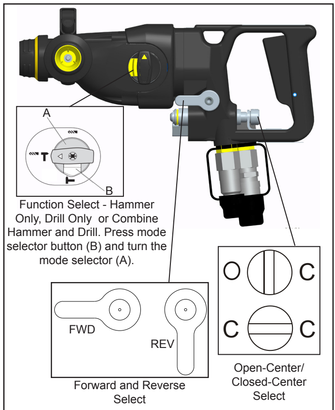
Figure 2. Operator Controls
