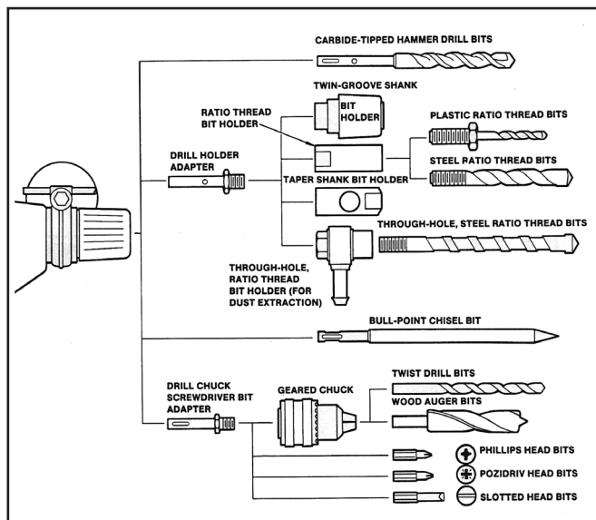
Figure 4. Hammer Drill Accessories
