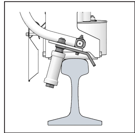
TYPICAL RAIL
